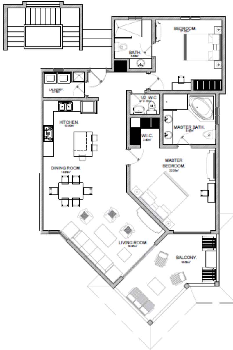
FLOOR PLAN . 1,644 Sq.Ft.
