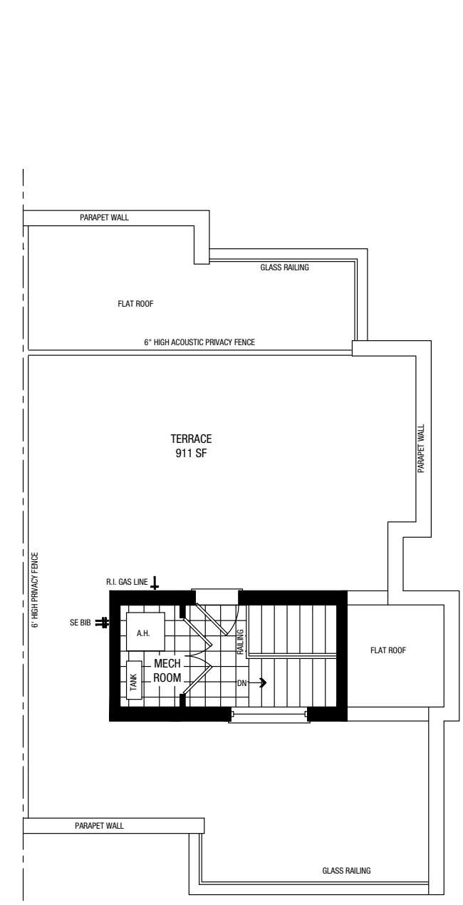
TERRACE BLOCK 13 UNIT 79 & BLOCK 21 UNIT 138 & 18 A
