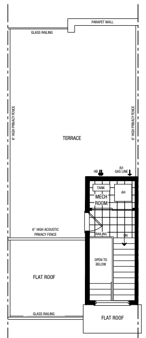
TERRACE BLOCK 14 UNIT 83 A
