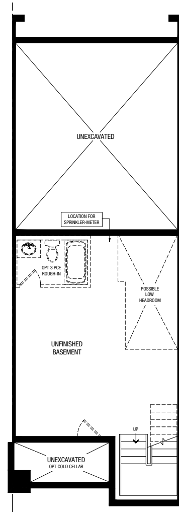
PARTIAL BASEMENT B
