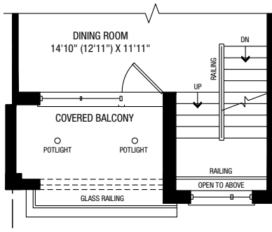
PARTIAL MAIN B
