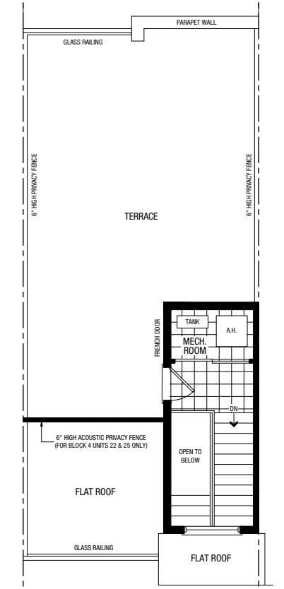
PARTIAL ROOF TERRACE B
