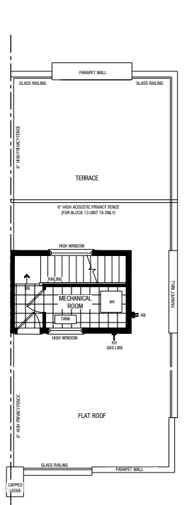
TERRACE BLOCK 14 UNIT 85 & BLOCK 13 UNIT 76 B
