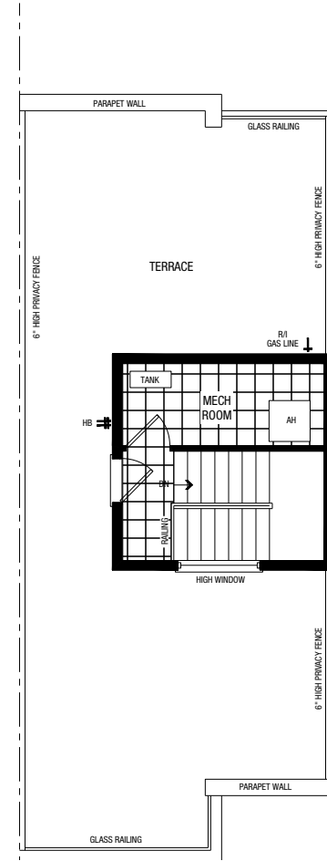
PARTIAL TERRACE B
