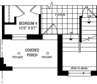
PARTIAL OPT. GROUND B
