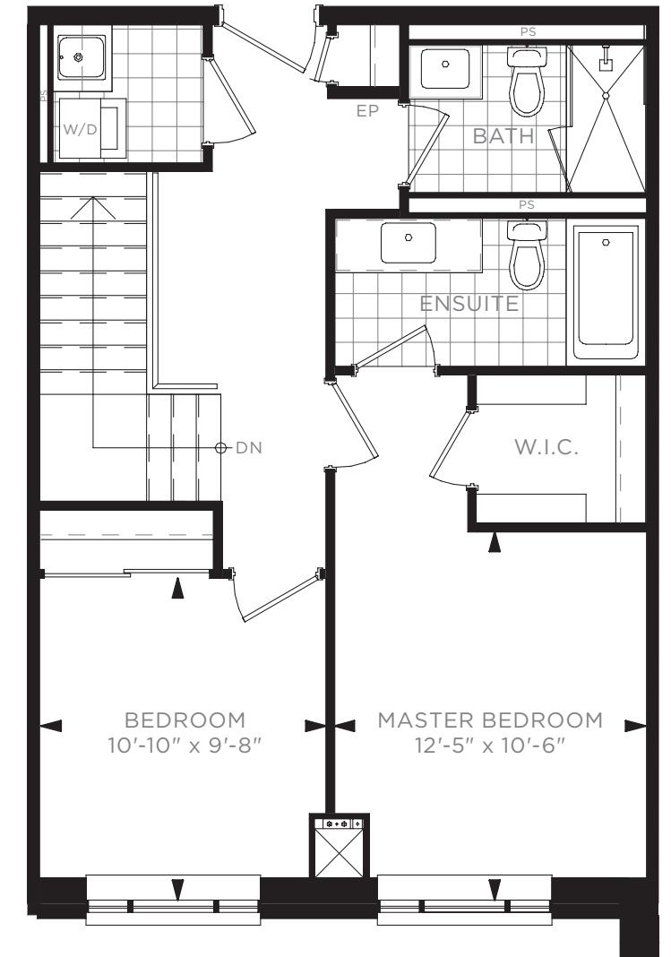
2ND FLOOR
