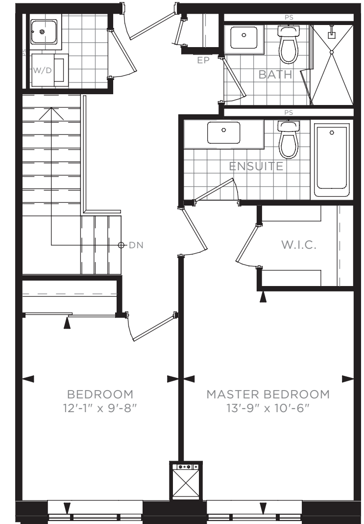
2ND FLOOR
