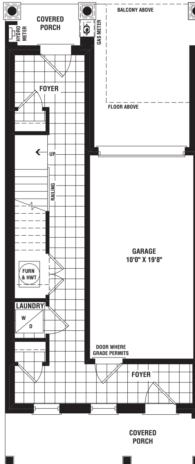
TH-1 MAIN FLOOR PLAN ELEV 'A' (INTERIOR END)
