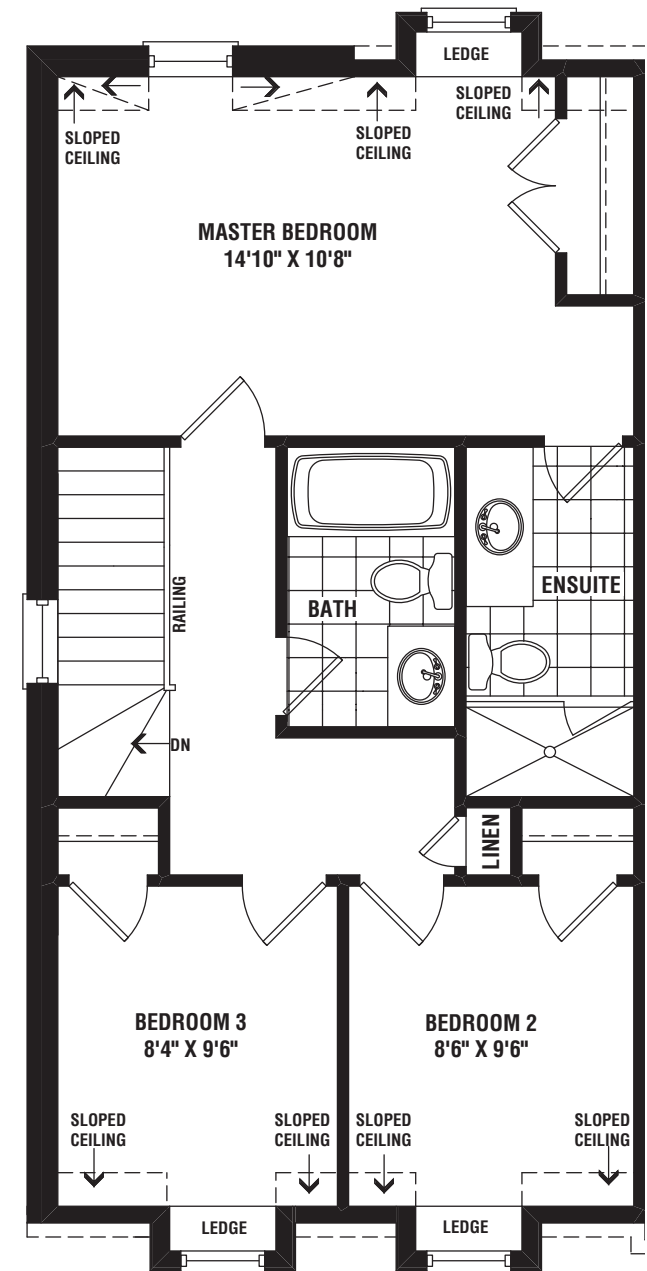
TH-1 THIRD FLOOR PLAN ELEV 'A' (INTERIOR END)
