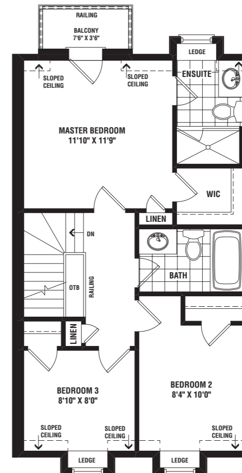
TH-3 THIRD FLOOR PLAN ELEV 'B' (INTERIOR END)
