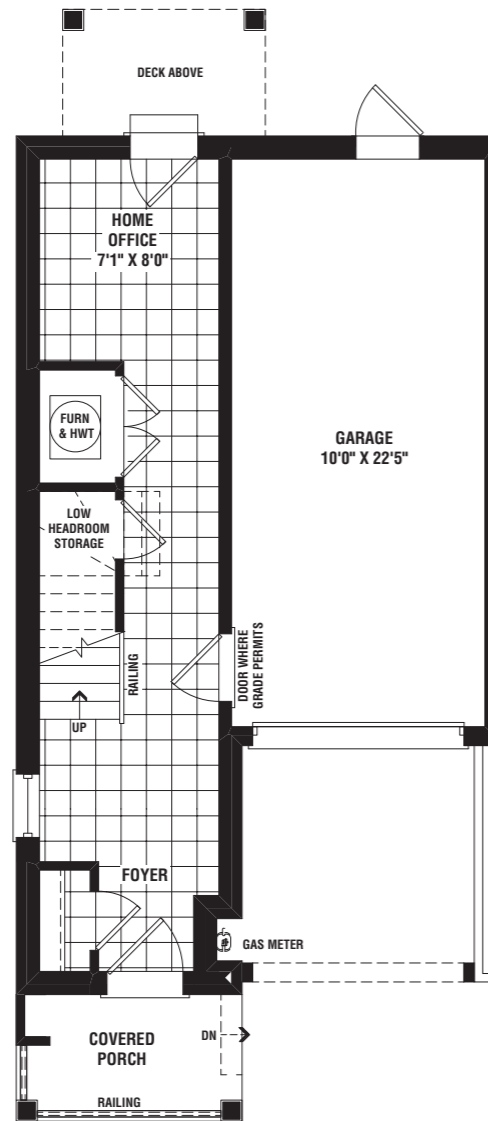
TH-3 MAIN FLOOR PLAN ELEV 'A' (EXTERIOR END)
