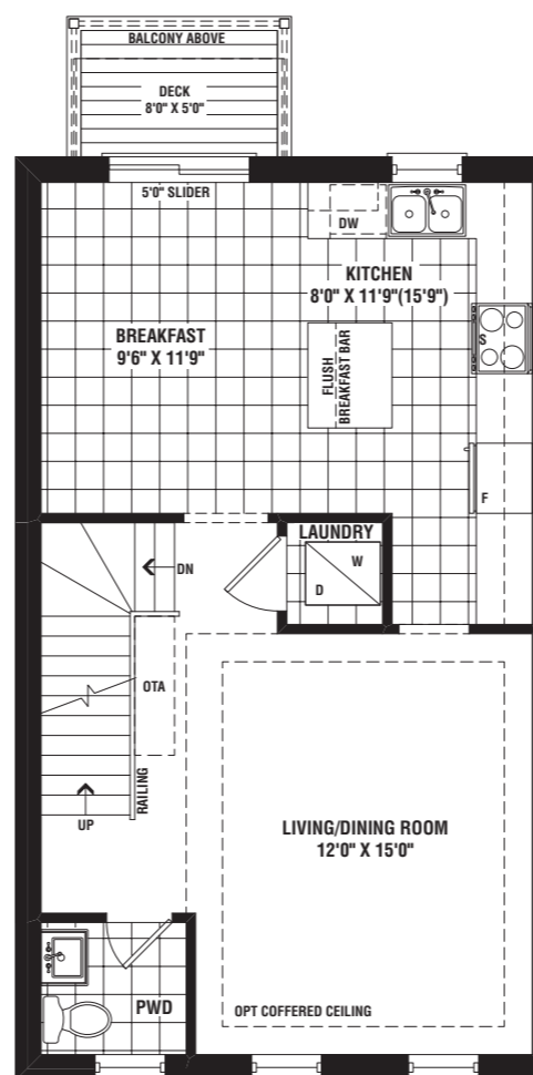
TH-3 SECOND FLOOR PLAN ELEV 'B' (INTERIOR END)
