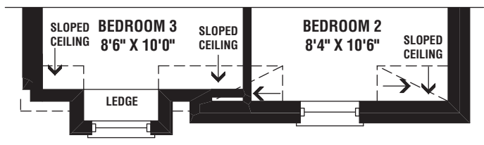
TH-1 THIRD FLOOR PLAN ELEV 'B' (EXTERIOR END)
