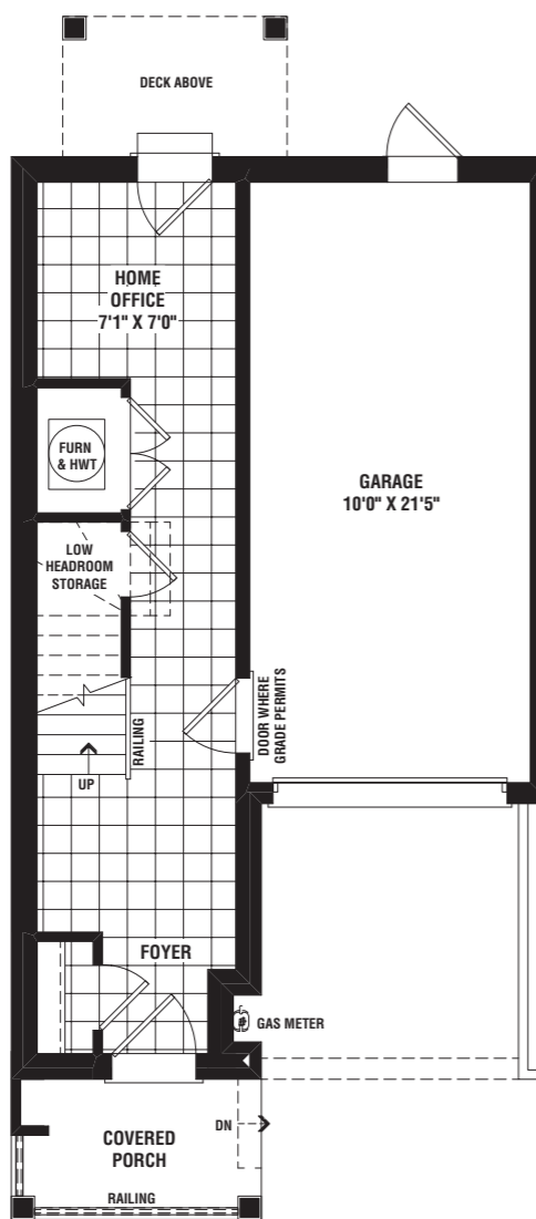
TH-3 MAIN FLOOR PLAN ELEV 'B' (INTERIOR END)
