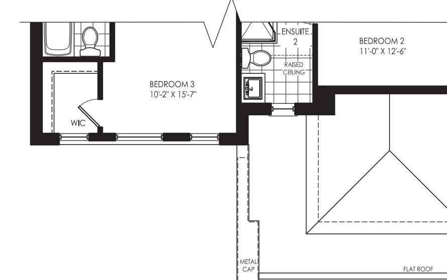
SECOND FLOOR ELEVATION C
