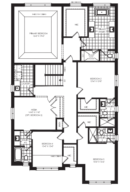
OPTIONAL SECOND FLOOR WITH MEDIA ROOM ELEVATION B
