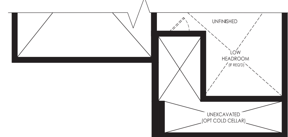
OPTIONAL FINISHED BASEMENT ELEVATION C
