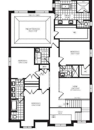
OPTIONAL SECOND FLOOR WITH MEDIA ROOM ELEVATION A
