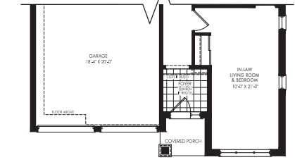
OPTIONAL GROUND FLOOR WITH IN-LAW LIVING ROOM & BEDROOM ELEVATION B
