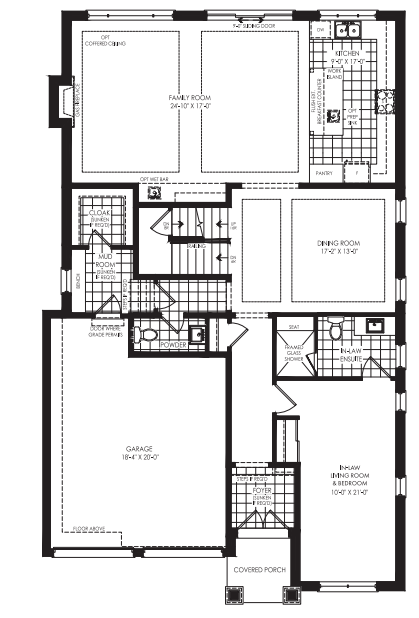
OPTIONAL GROUND FLOOR WITH IN-LAW LIVING ROOM & BEDROOM ELEVATION B
