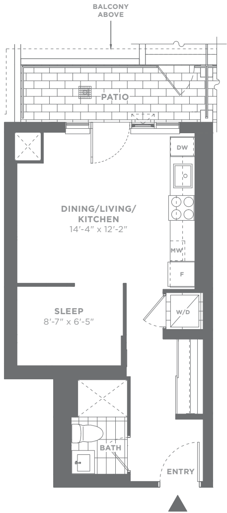
BUILDING A
