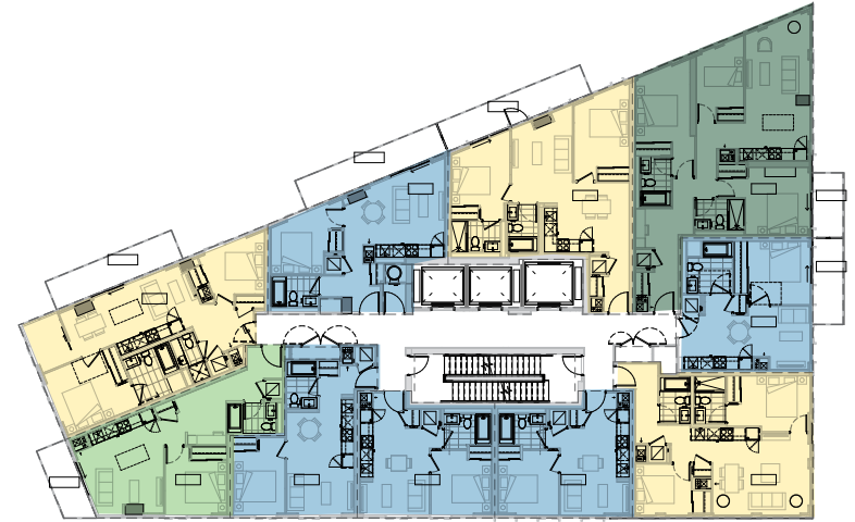
8th Floor
