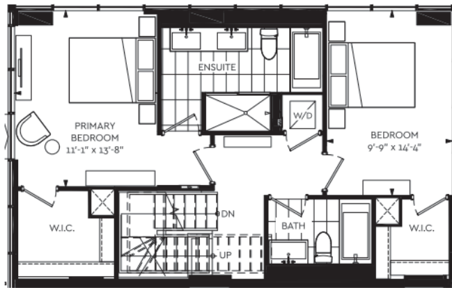
UPPER FLOOR
