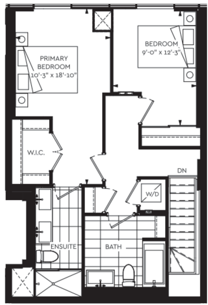
UPPER FLOOR
