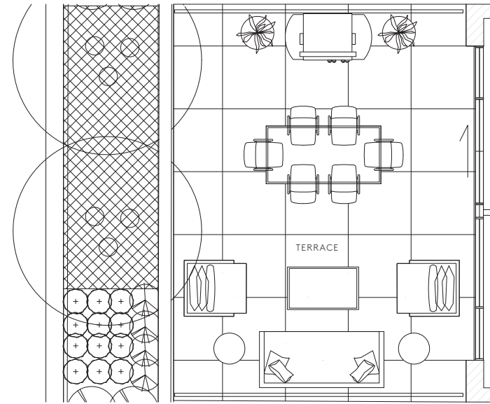
2ND FLOOR - 318 SQ.FT.
