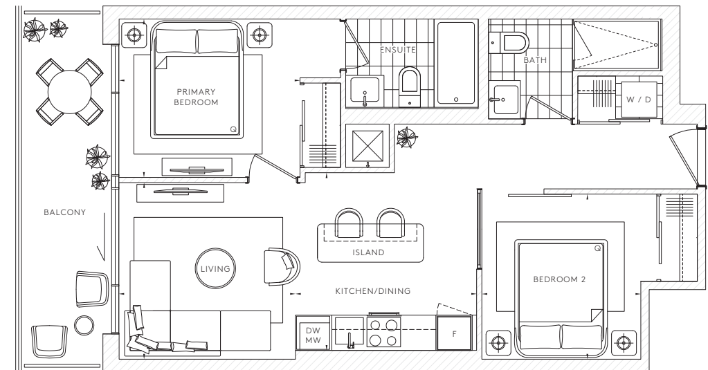
3RD - 5TH FLOOR - 98 SQ.FT.
