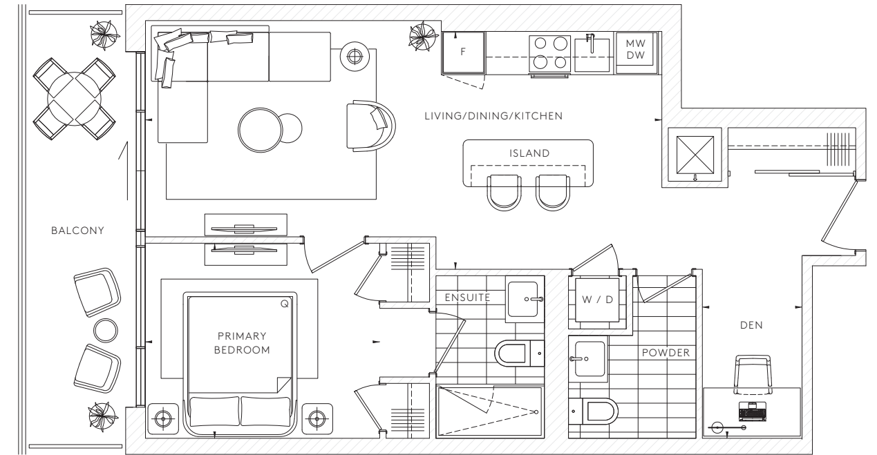
6TH FLOOR - 98 SQ.FT. 7TH - 12TH FLOOR - 100 SQ.FT.
