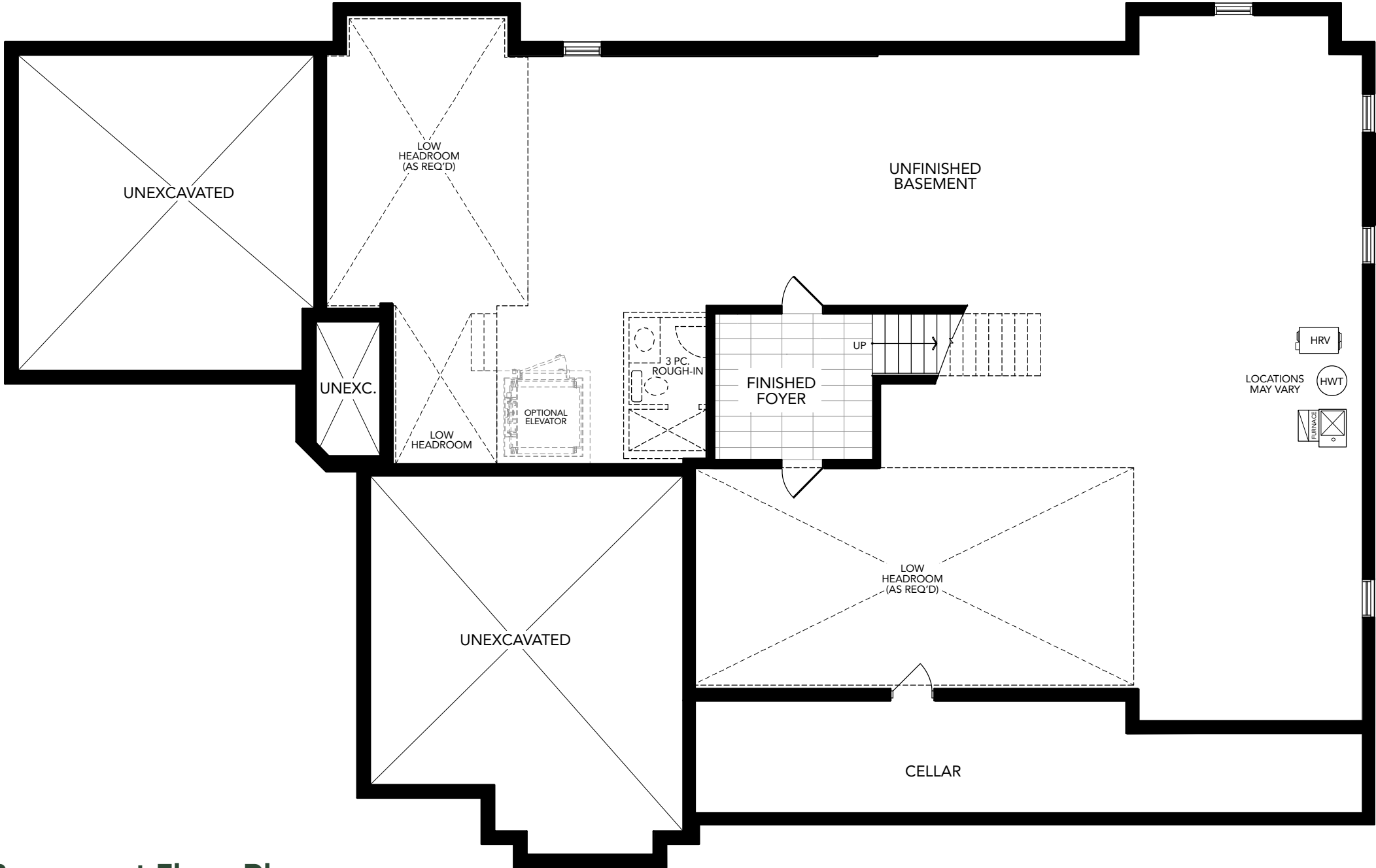
Basement Floor Plan Elevation B
