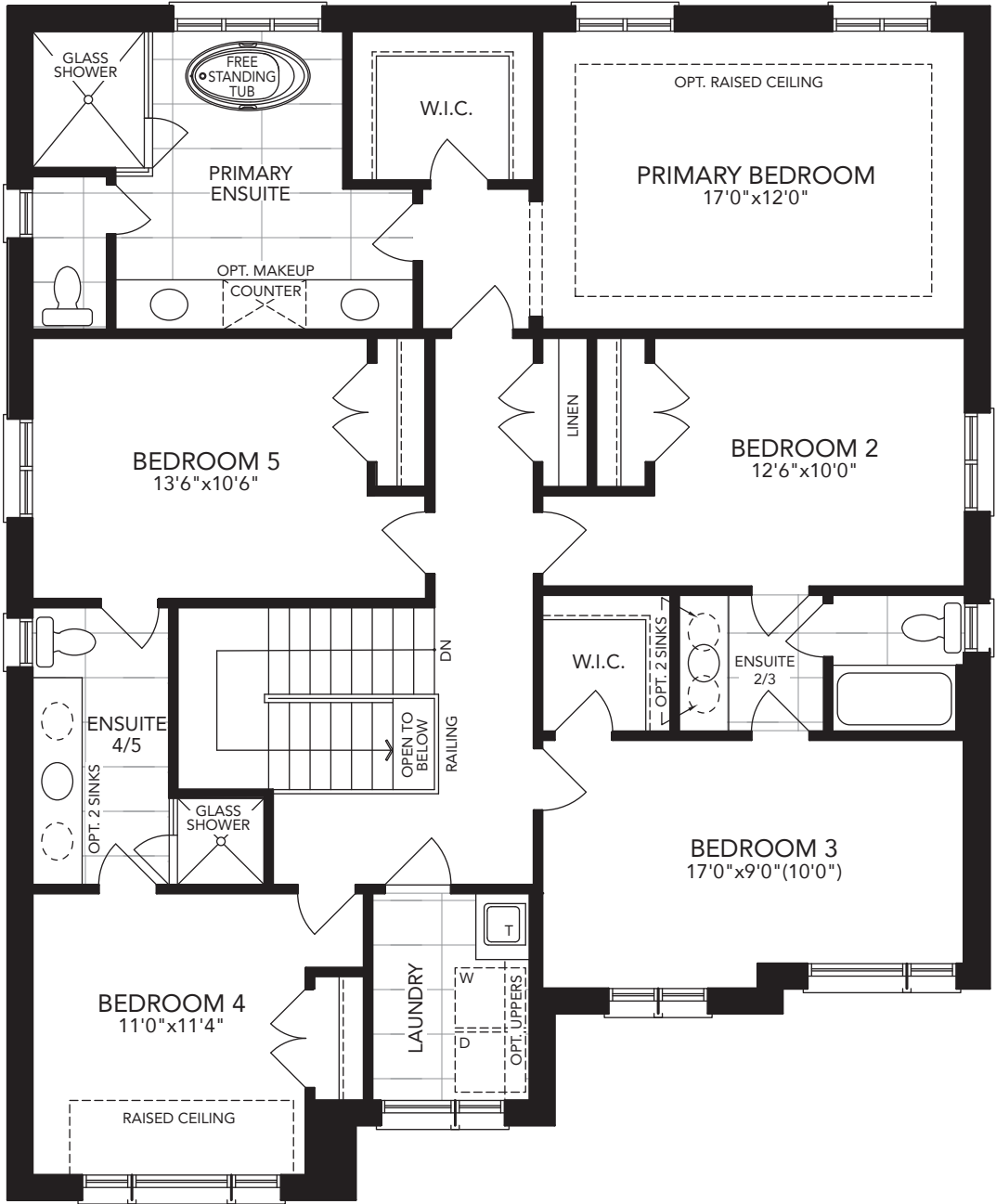
Opt. Second Floor Plan with 5 Bedroom Elevation A
