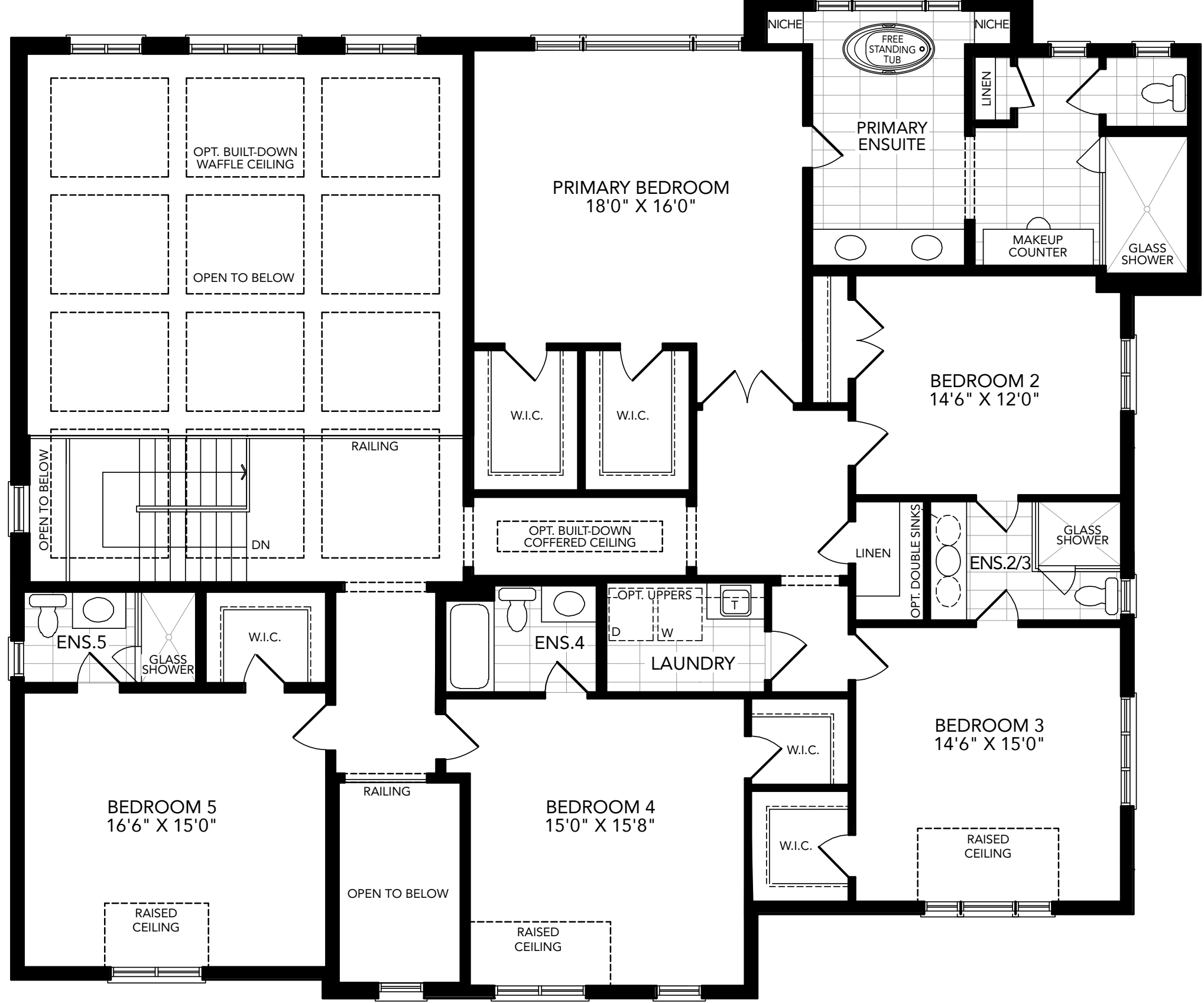
Second Floor Plan Elevation B
