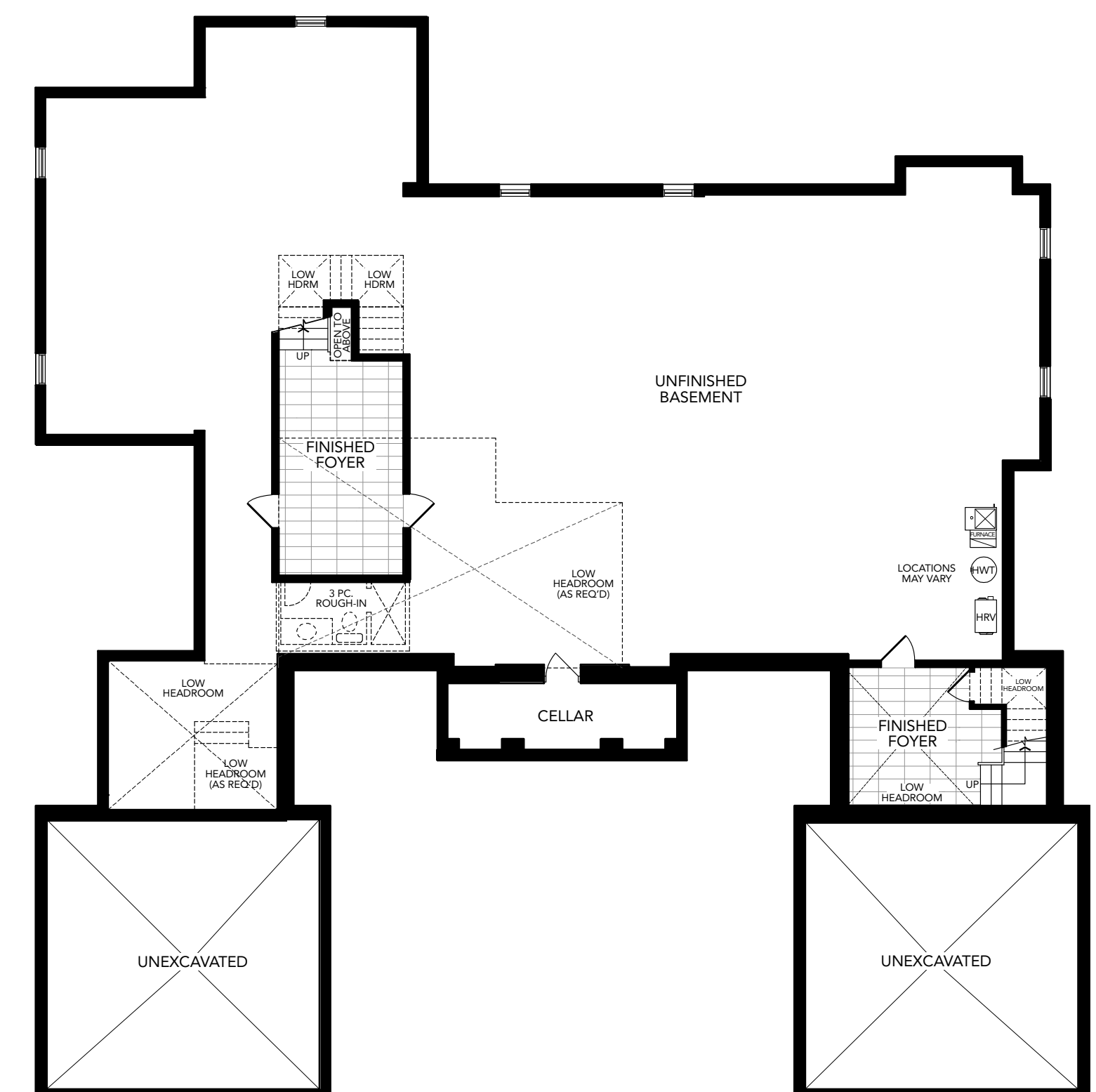
Basement Plan Elevation A
