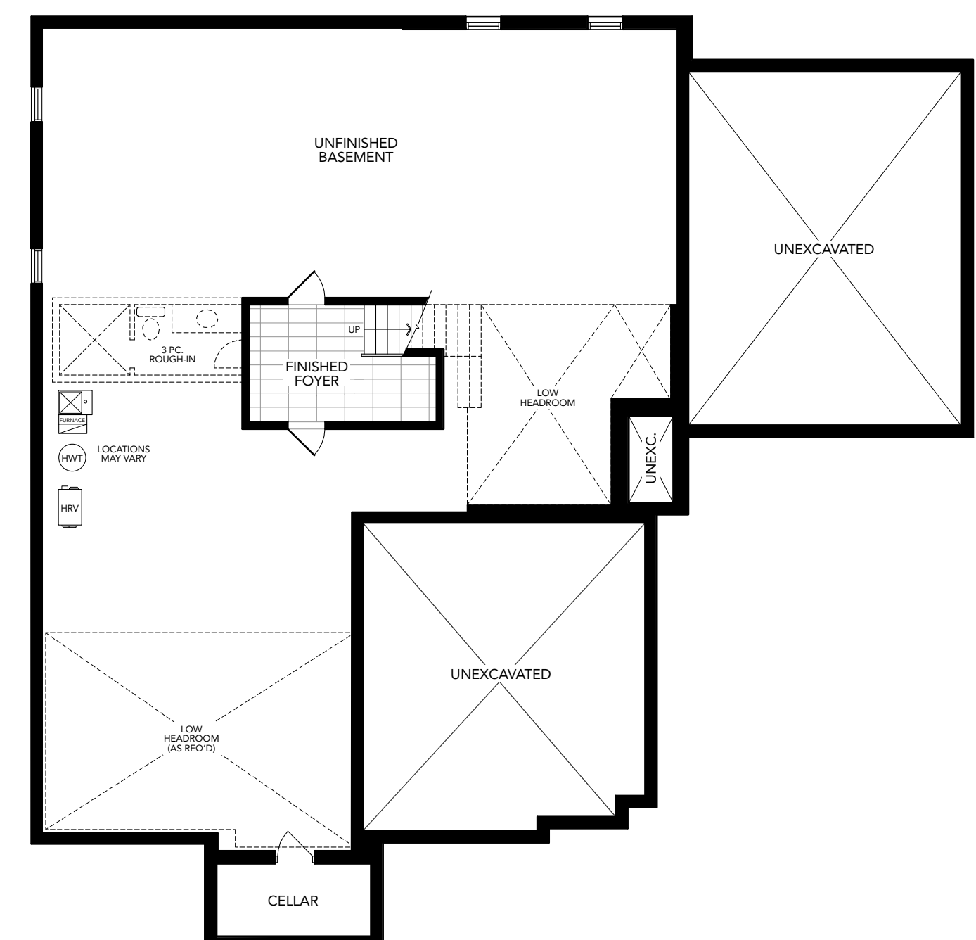
Basement Floor Plan Elevation B
