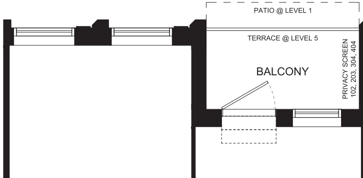
UNIT PART PLAN @ 519, 619, 719
