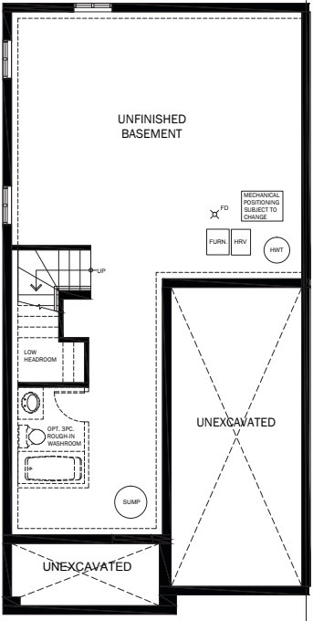
Basement Elevation A & B
