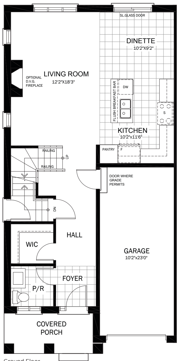
Ground Floor Elevation A & B
