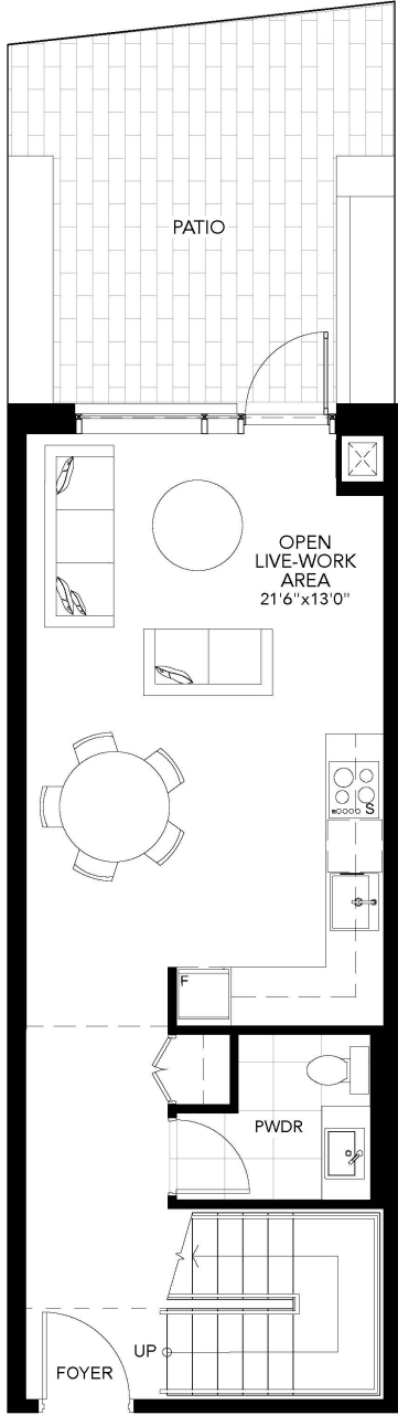
1 ST LEVEL
