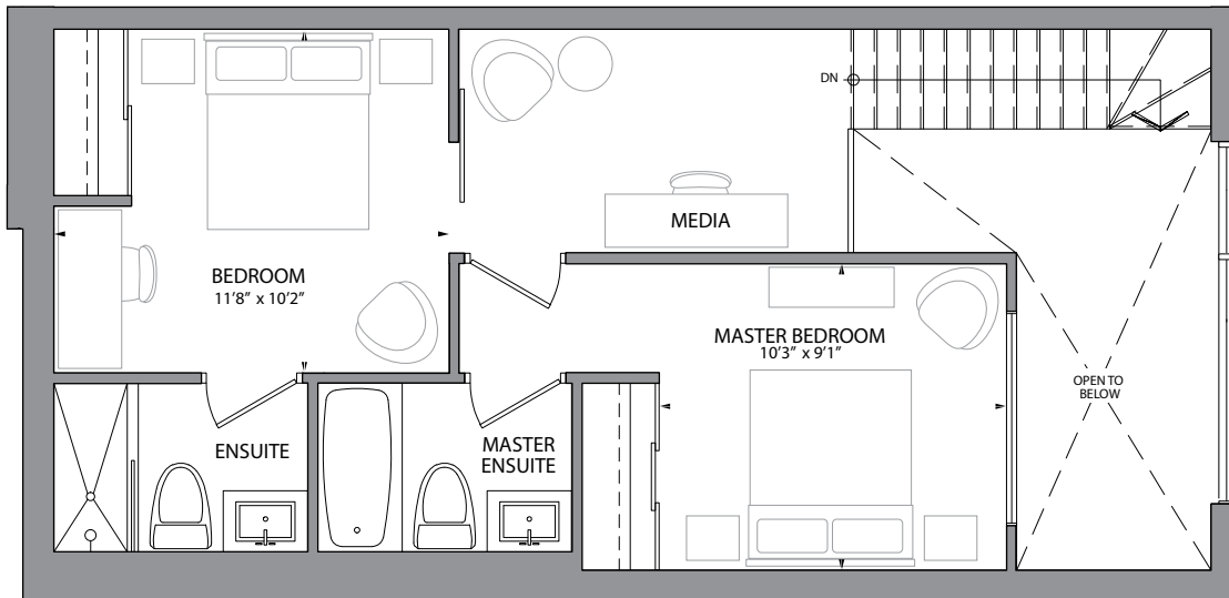
LOFT LEVEL
