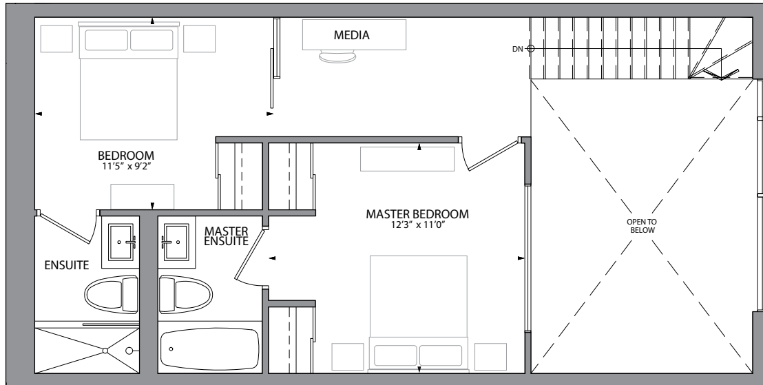
LOFT LEVEL
