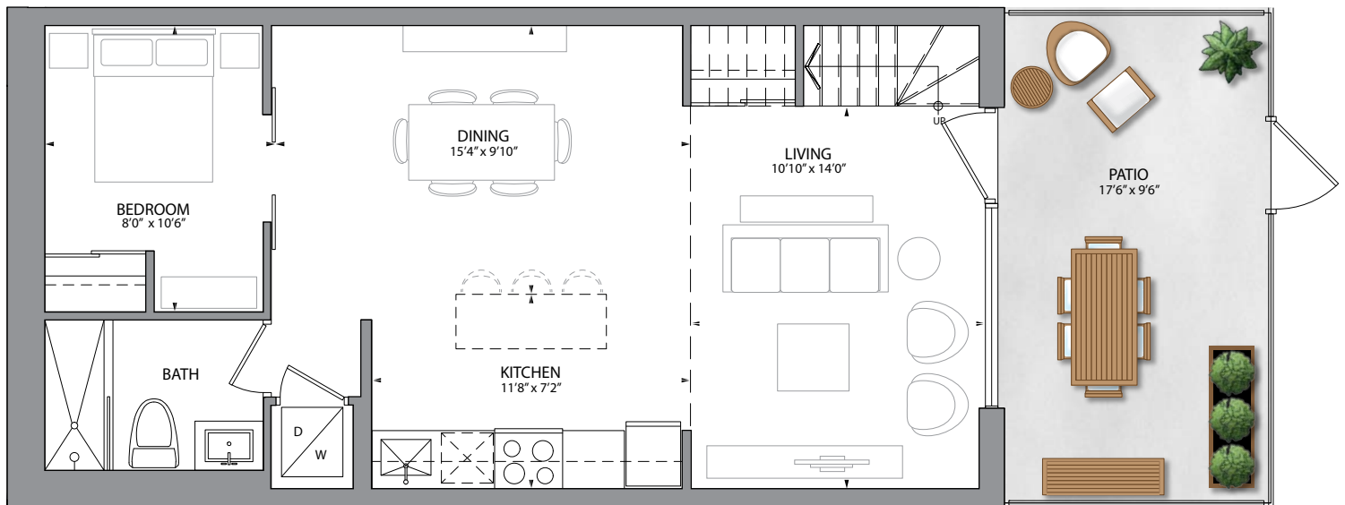
MAIN LEVEL
