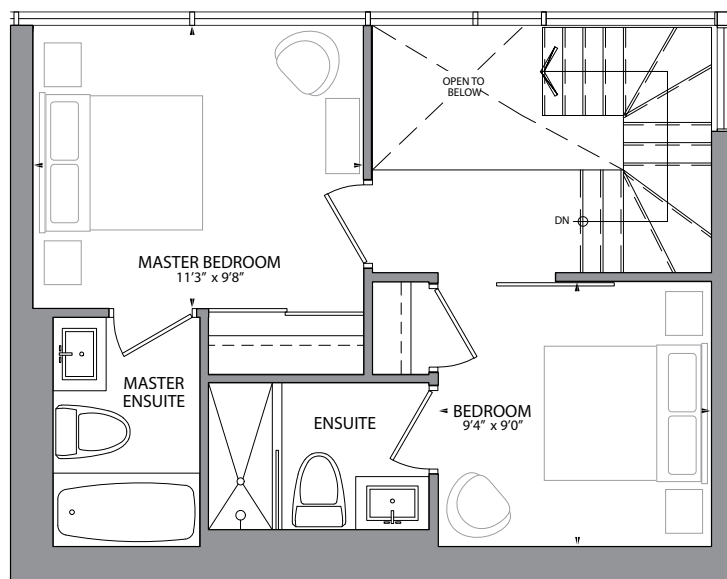
LOFT LEVEL
