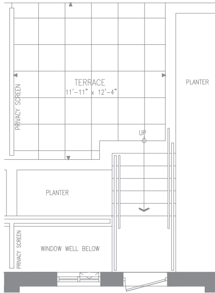
Terrace Area
