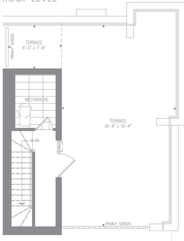
ROOF LEVEL
