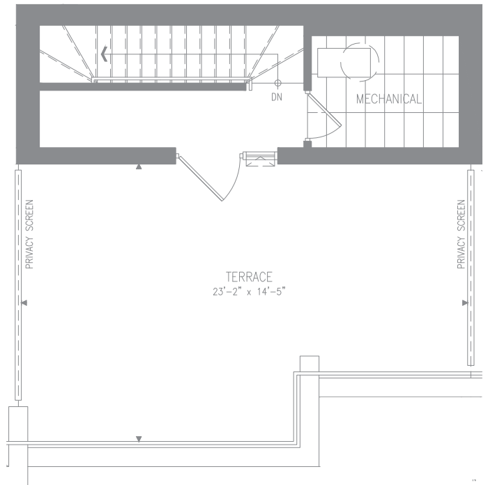
ROOF LEVEL
