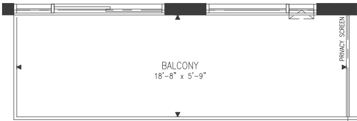
Balcony at Levels 2 to 10 - Suite 30
