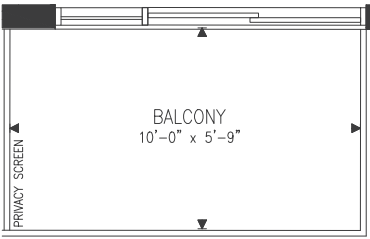
Balcony at Levels 3/5/7/9 - Suite 32
