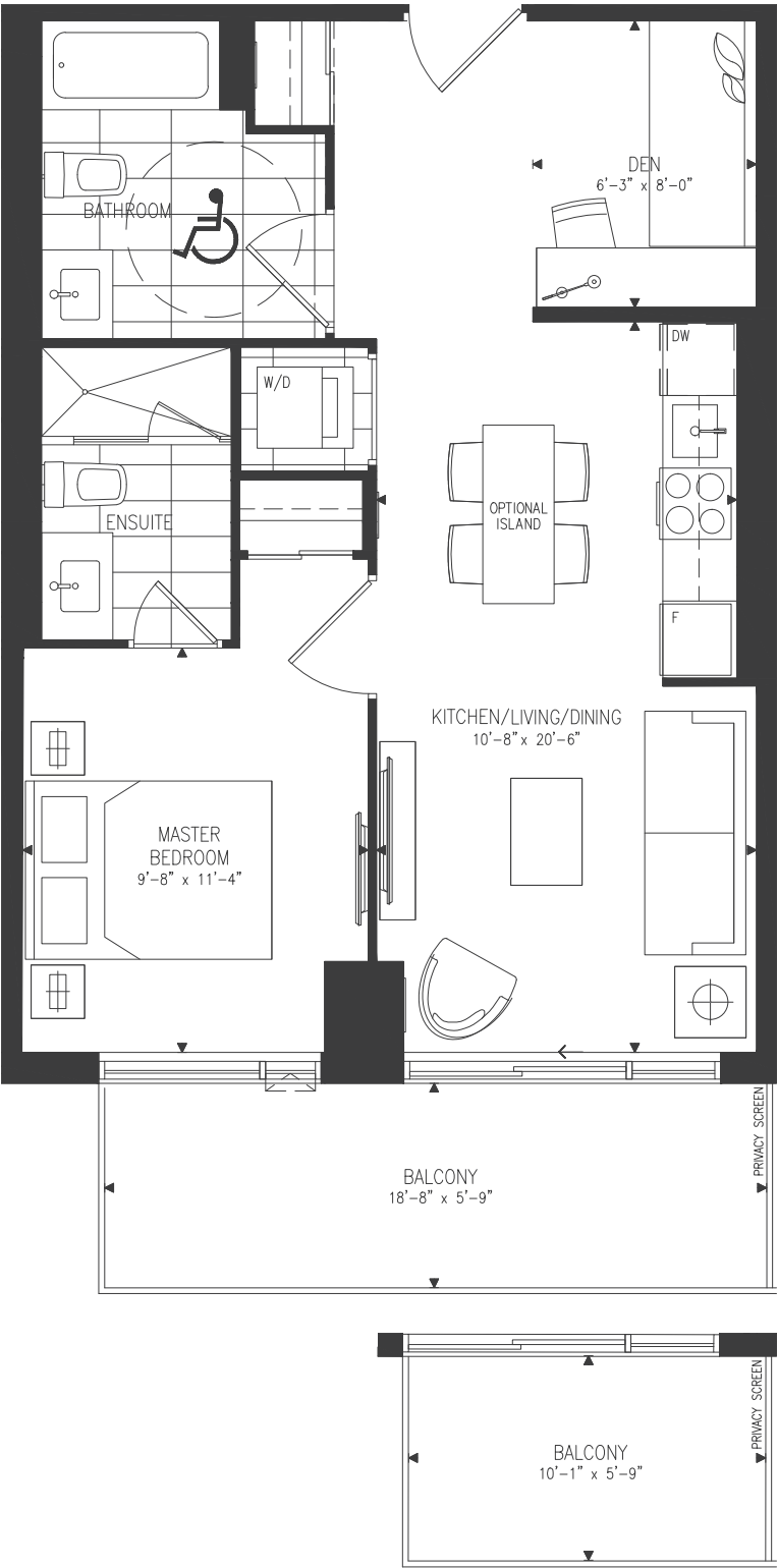
Balcony at Levels 3/5/7/9
