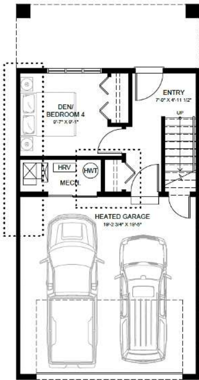
GROUND LEVEL ±210 SQ. FT.
