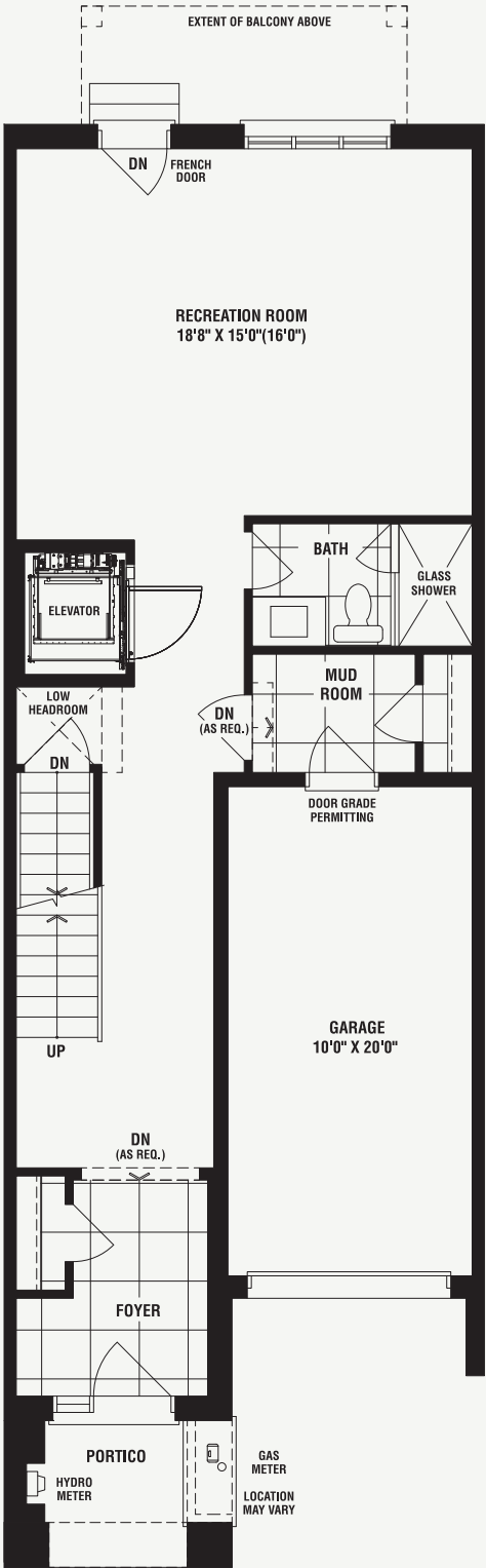
GROUND FLOOR PLAN ELEV. 'A' ELEVATOR CONDITION
