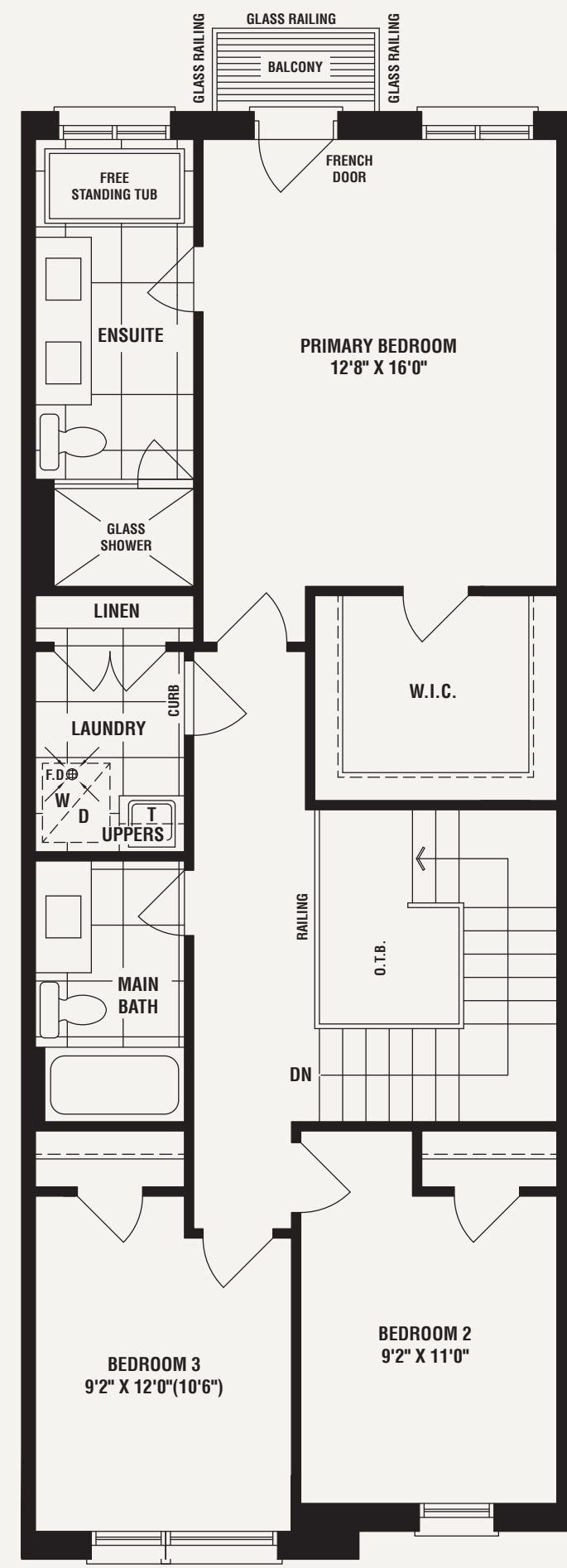
OPT. UPPER FLOOR PLAN ELEV. 'A'
