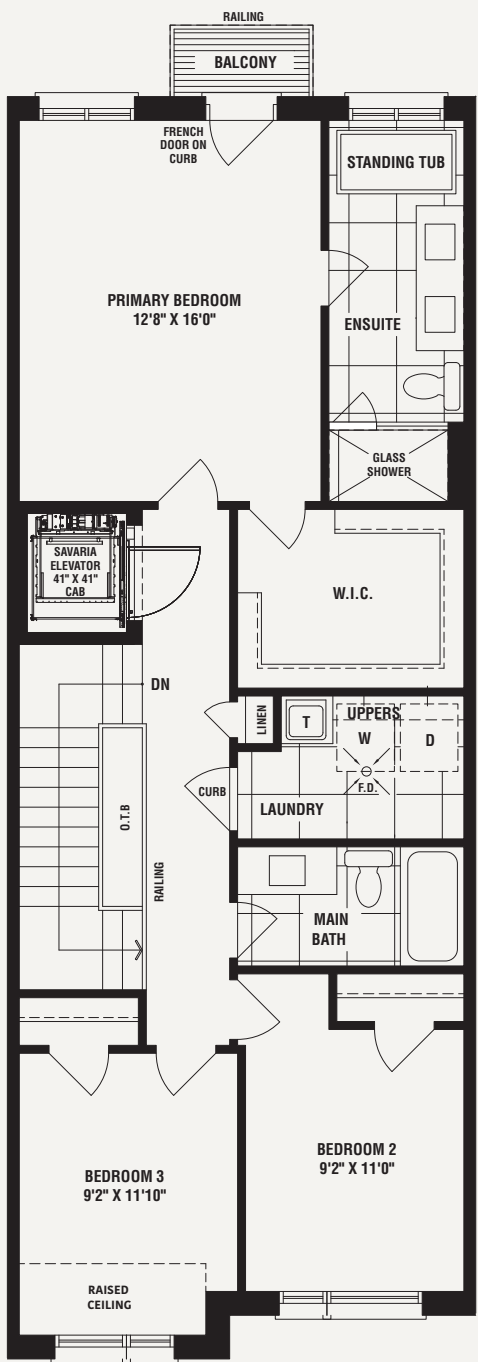
UPPER FLOOR PLAN ELEV. 'A' ELEVATOR CONDITION
