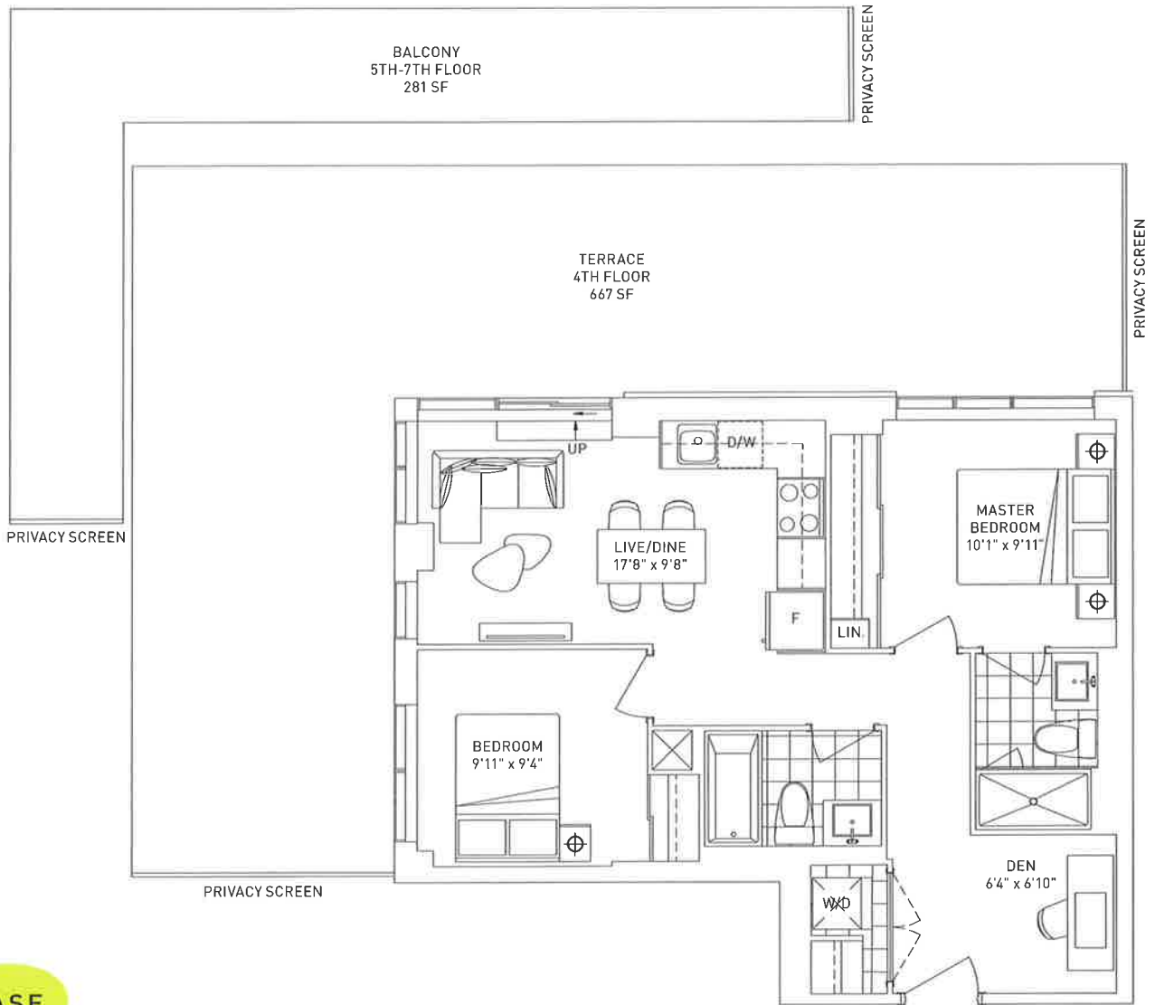
5th-7th floor
