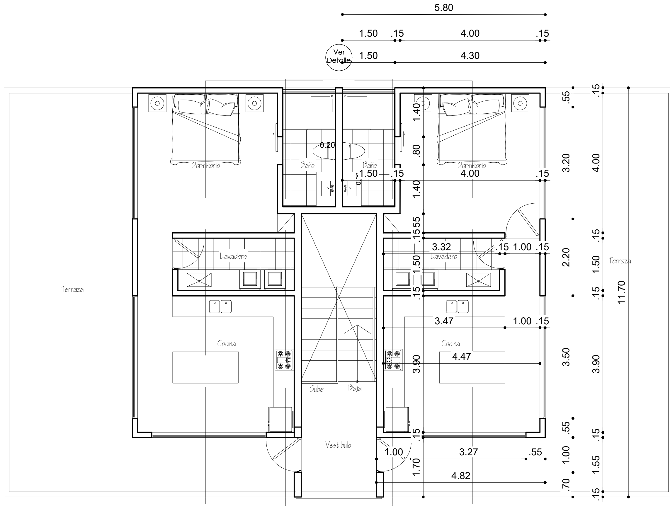
PENTHOUSE 1-BED FLOORPLAN - LEVEL 4
