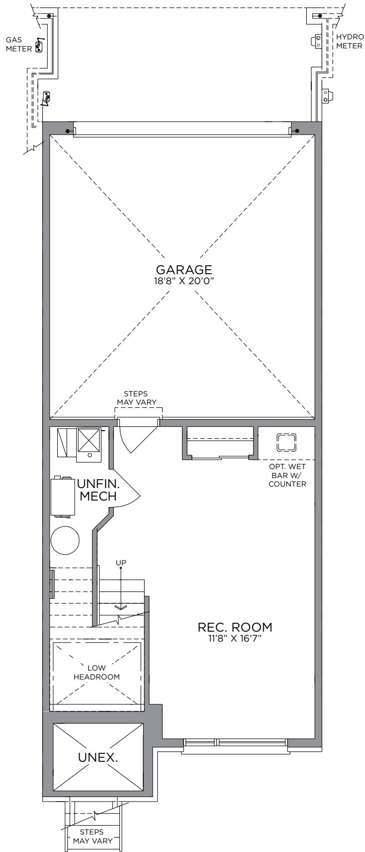
GROUND FLOOR PLAN ELEV. A
