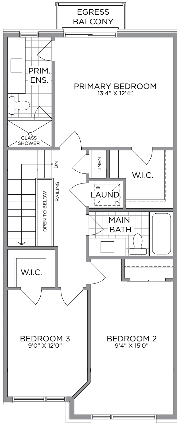
UPPER FLOOR PLAN ELEV. A
