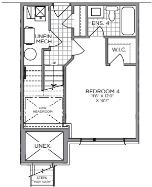
PART. OPT. GROUND FLOOR PLAN W/ 4 BEDROOM ELEV. A
