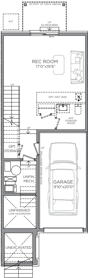
GROUND FLOOR PLAN ELEV. A FINISHED
