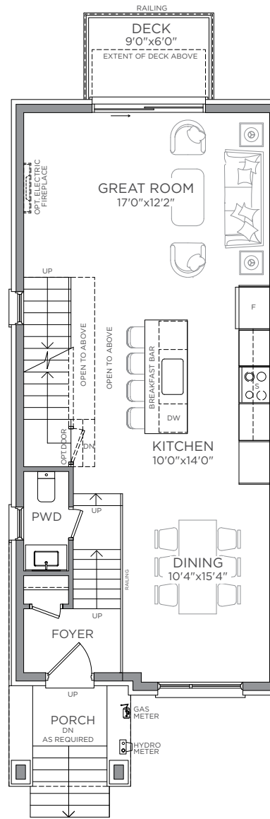
MAIN FLOOR PLAN ELEV. A
