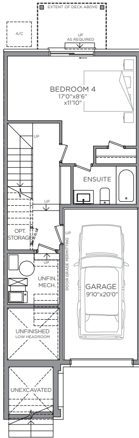
GROUND FLOOR PLAN ELEV. A FINISHED OPT. 2
