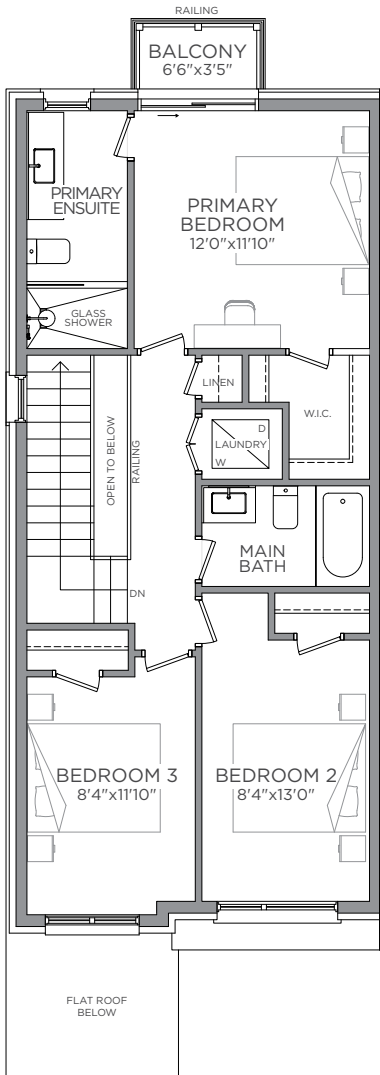
UPPER FLOOR PLAN ELEV. A
