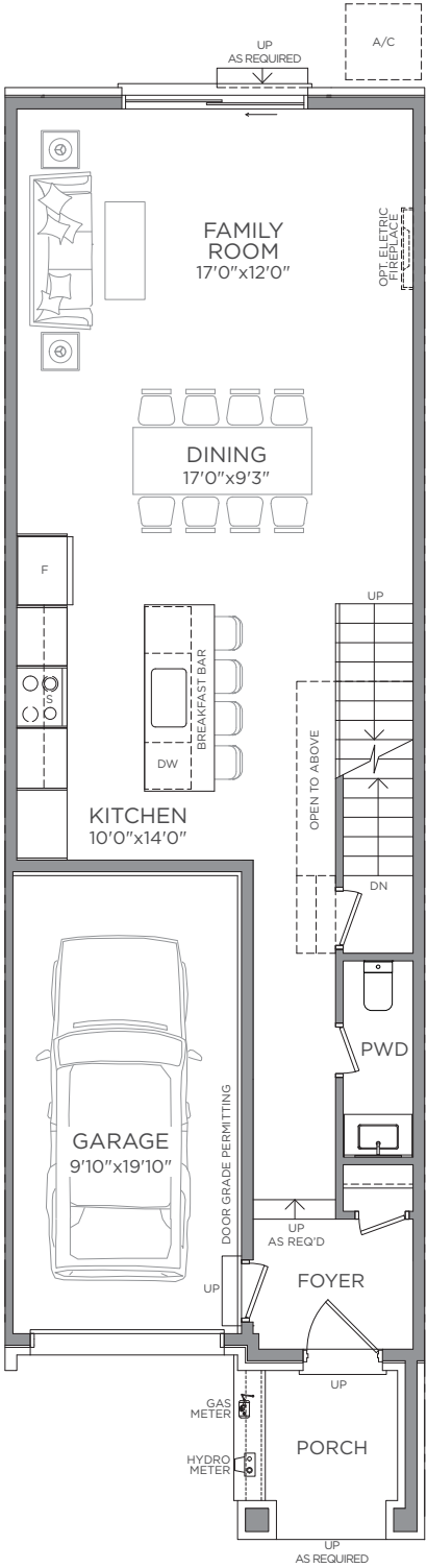
MAIN FLOOR PLAN
