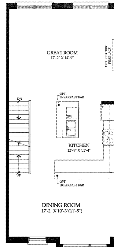
PART SECOND FLOOR OPT. KITCHEN
